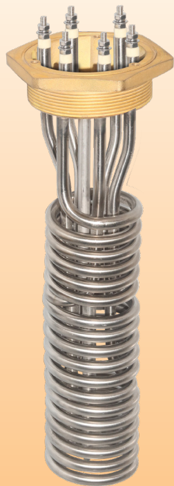
带2½" BSPP和M77×2接头
